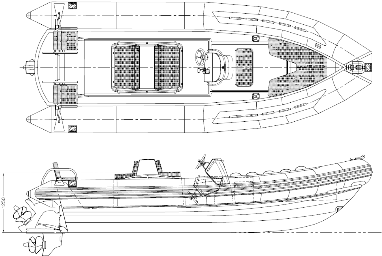
Figure 1 Suggested low profile layout for typical tender use
